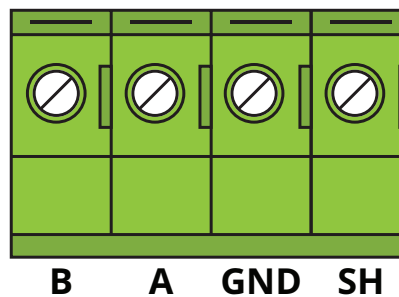
Figure 3-3 - MODBUS/Sensor Terminal Block
